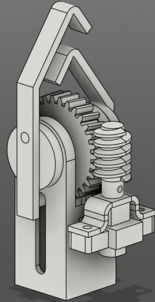
Assembled View of Final Prototype
