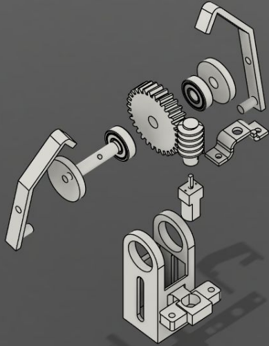
Exploded View of Final Prototype
