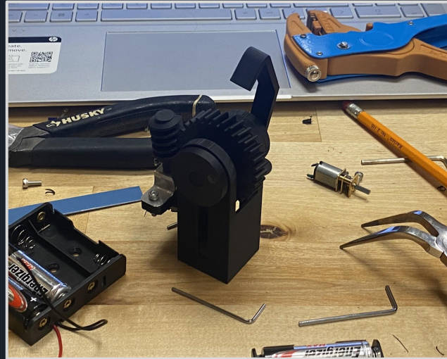
Assembly process featuring gear box and internal mechanisms
